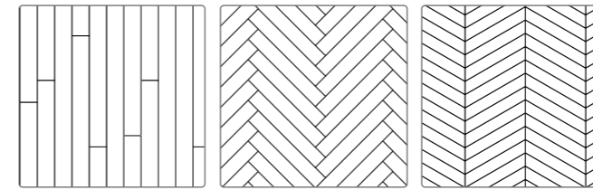
A CORRERE REGULAR INSTALLATION SPINA ITALIANA 90° ITALIAN HERRINGB. 90° PUNTO D'UNGERIA 60° CHEVRON PATTERN 60°
